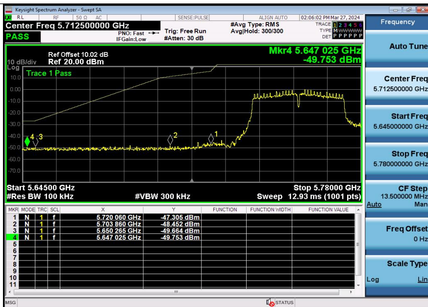
11N40SISO-Ant3-5755-PASS
