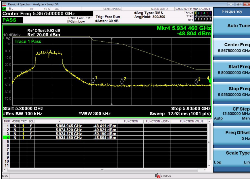
11AC20SISO-Ant3-5825-PASS
