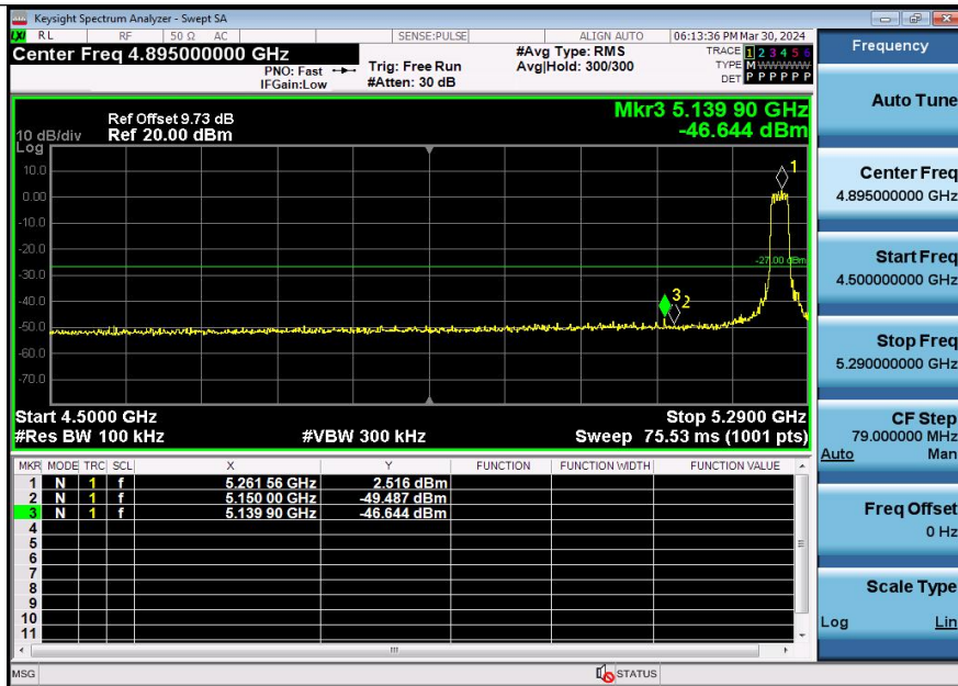
11AX20SISO-Ant3-5260-PASS
