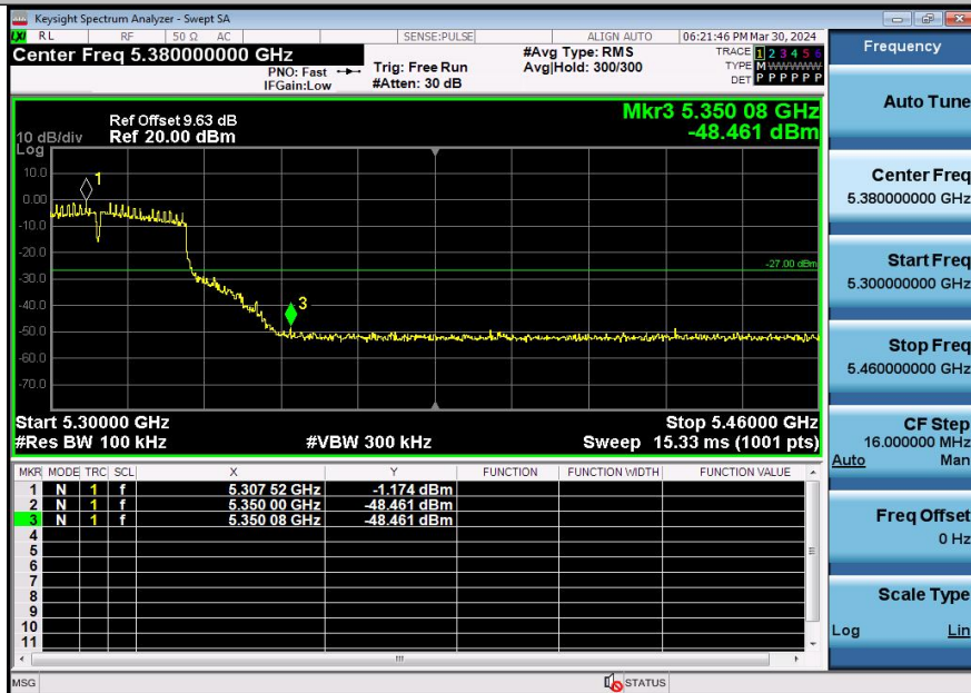
11AX40SISO-Ant3-5310-PASS
