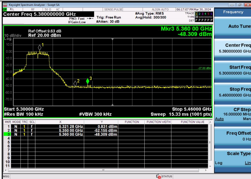
11AX20SISO-Ant3-5320-PASS
