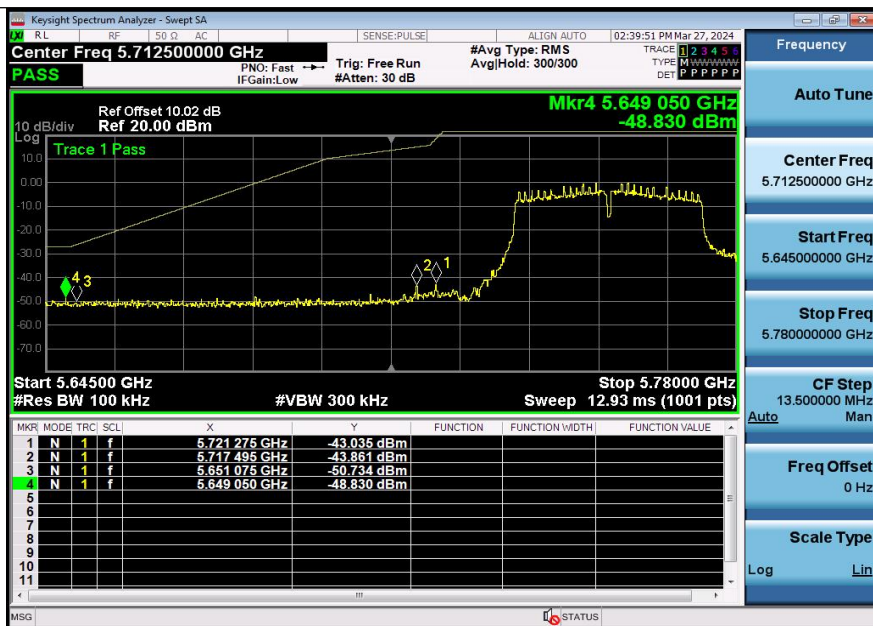
11AC40SISO-Ant3-5755-PASS
