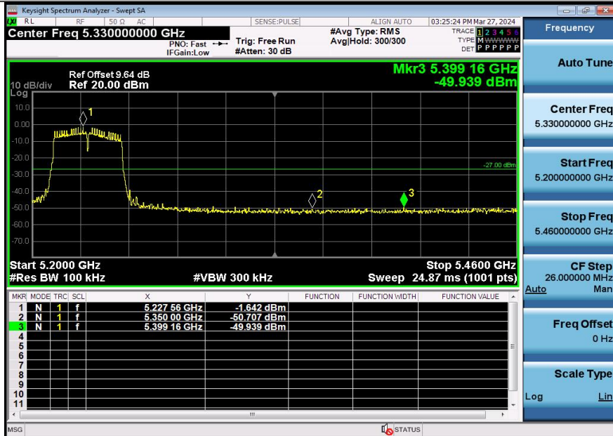
11AX40SISO-Ant3-5230-PASS
