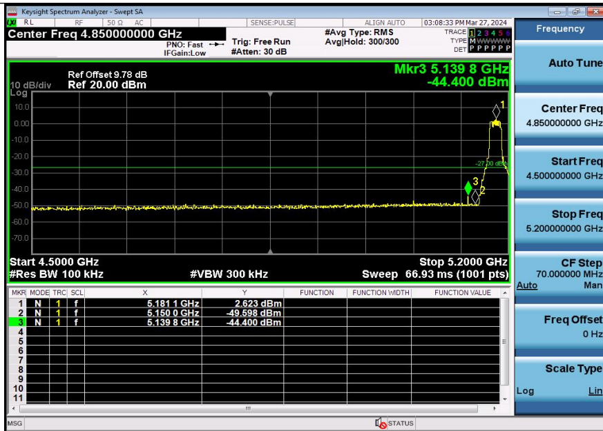
11AX20SISO-Ant3-5180-PASS
