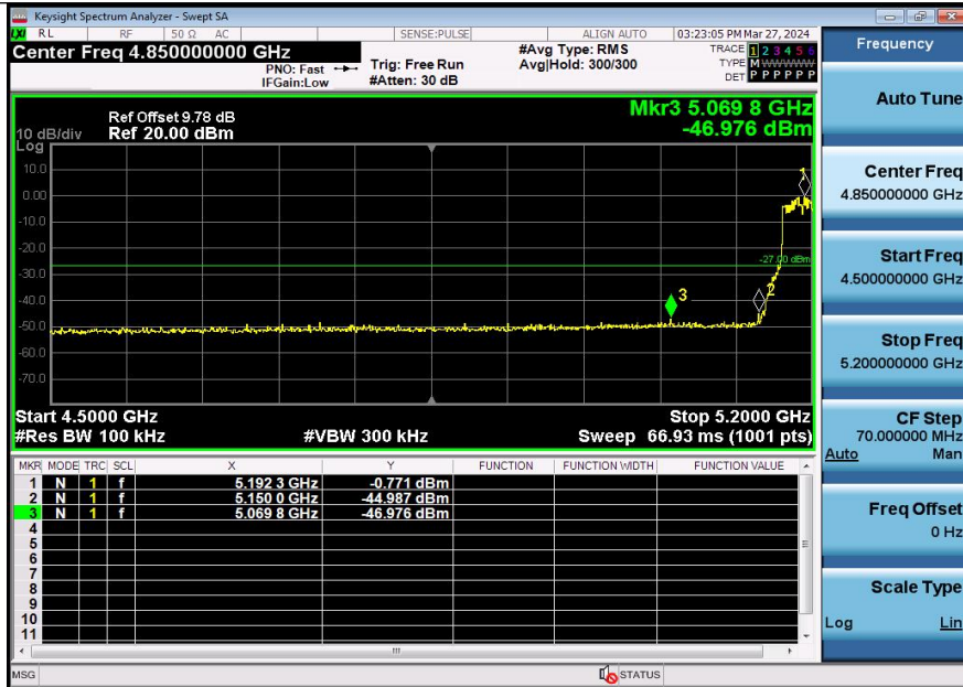
11AX40SISO-Ant3-5190-PASS
