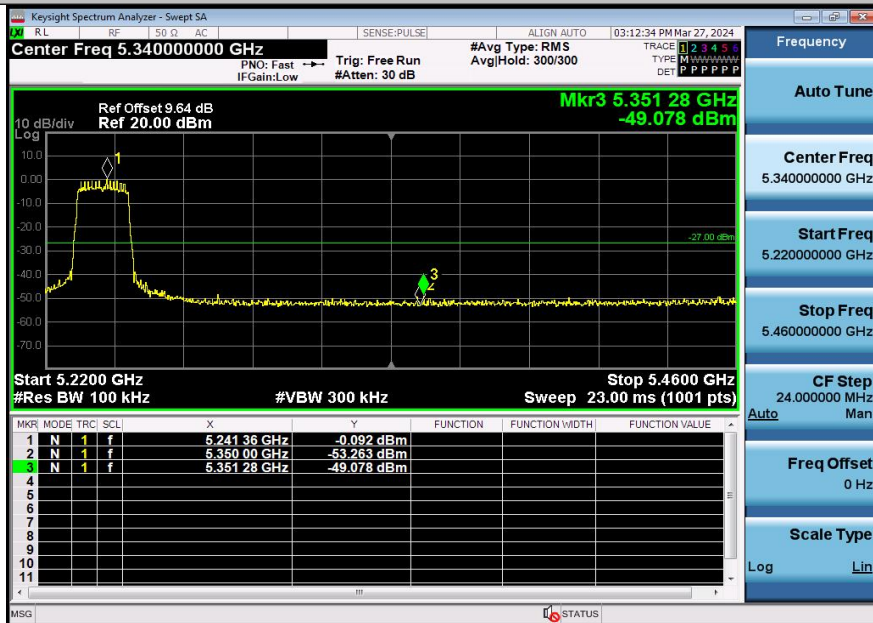
11AX20SISO-Ant3-5240-PASS
