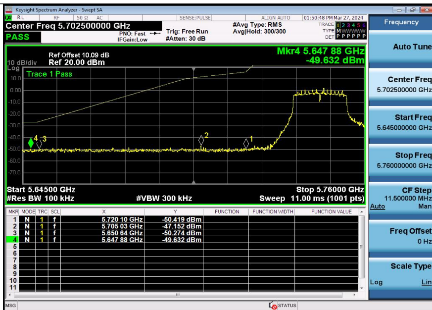
11N20SISO-Ant3-5745-PASS
