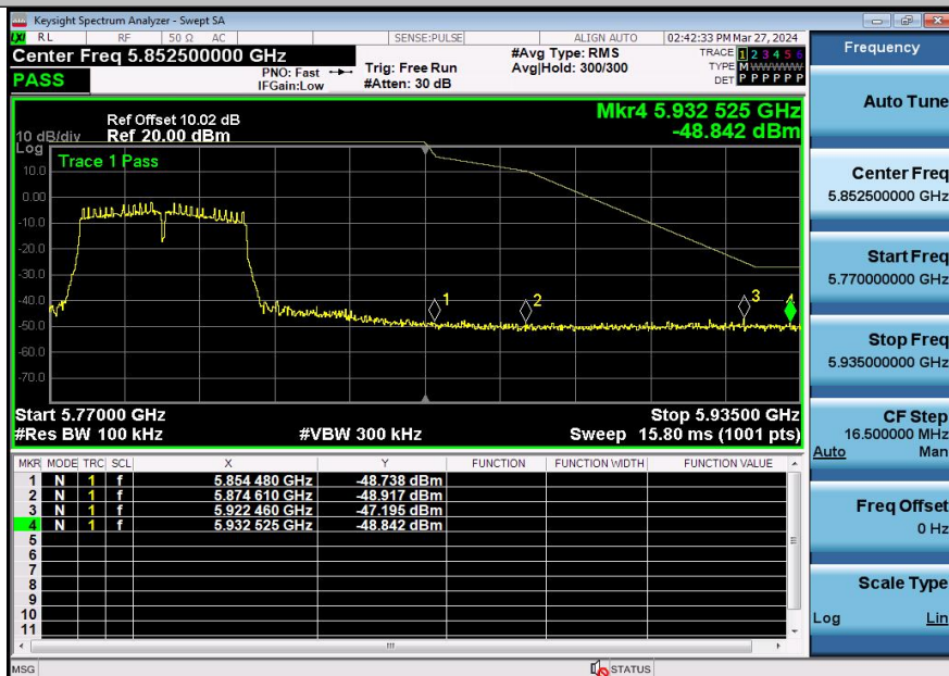
11AC40SISO-Ant3-5795-PASS
