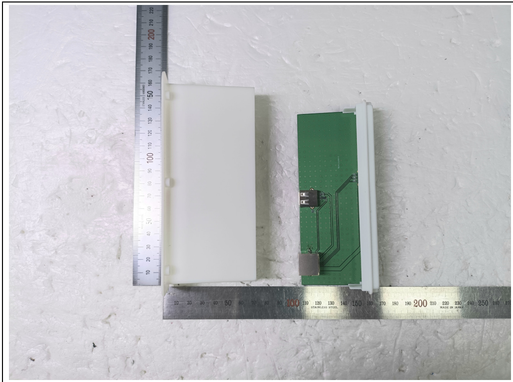
<B Board>
