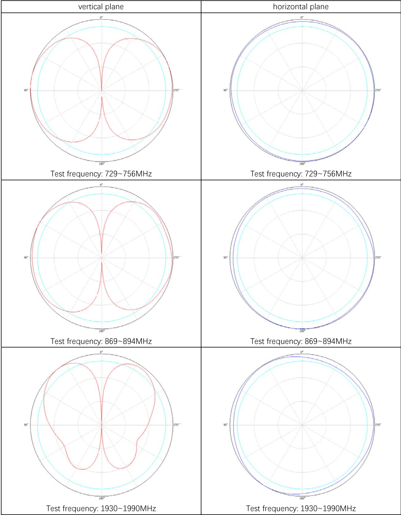
Dome antenna ambient temperature pattern
