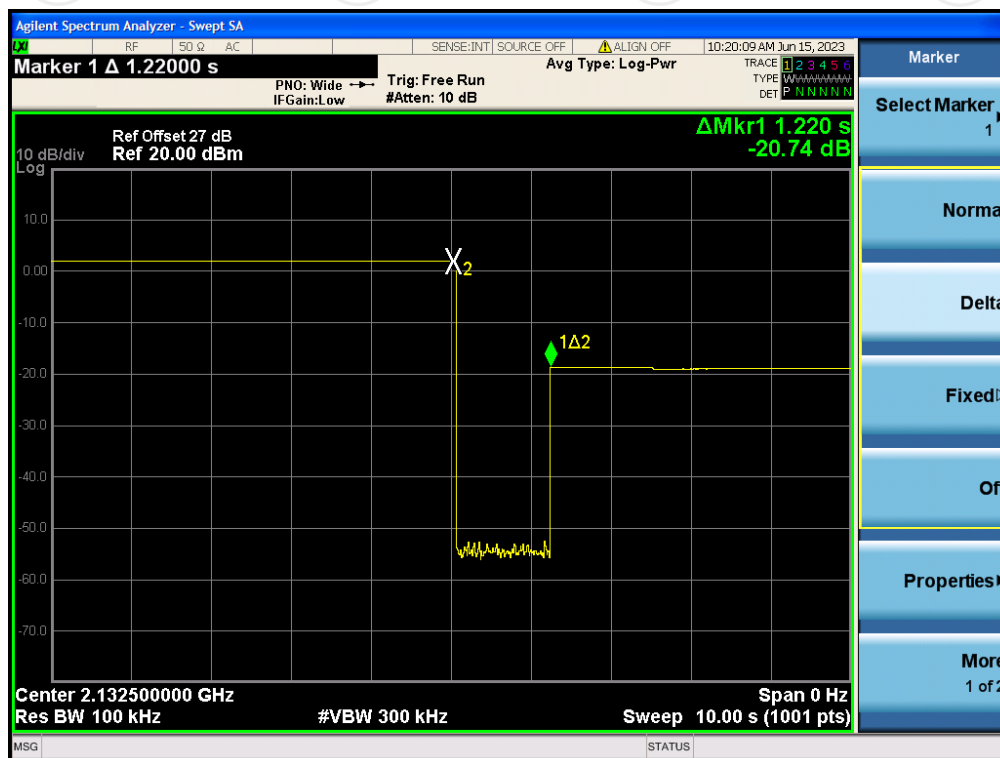
Band 4
