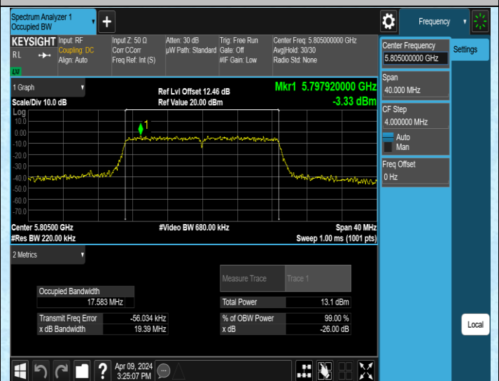
11N20SISO-Ant2-5805
