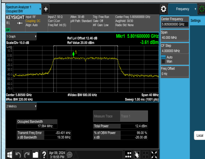
11N20SISO-Ant1-5805
