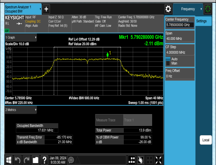
11N20MIMO-Ant4-5785
