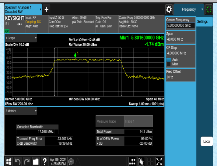
11N20MIMO-Ant4-5805
