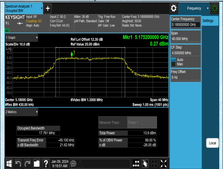
11N20MIMO-Ant4-5180
