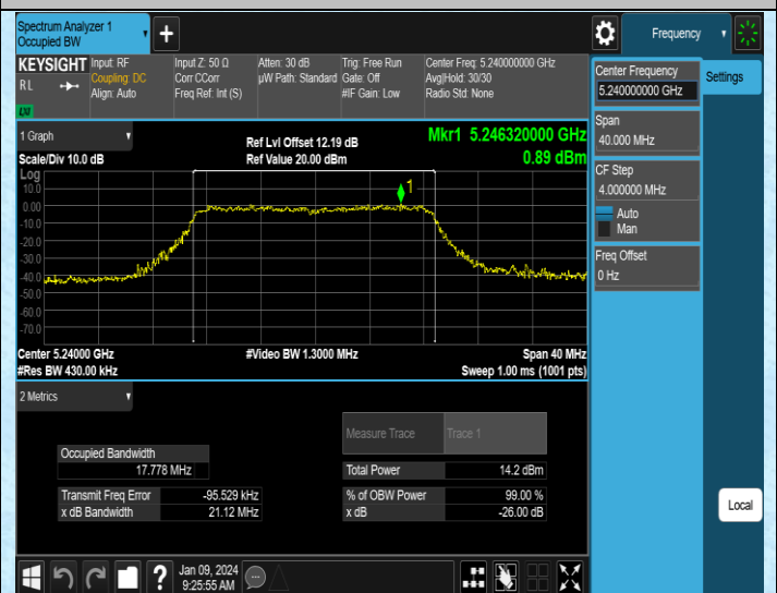
11N20MIMO-Ant4-5240
