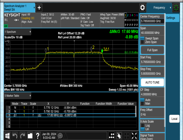
11N20MIMO-Ant4-5785-PASS
