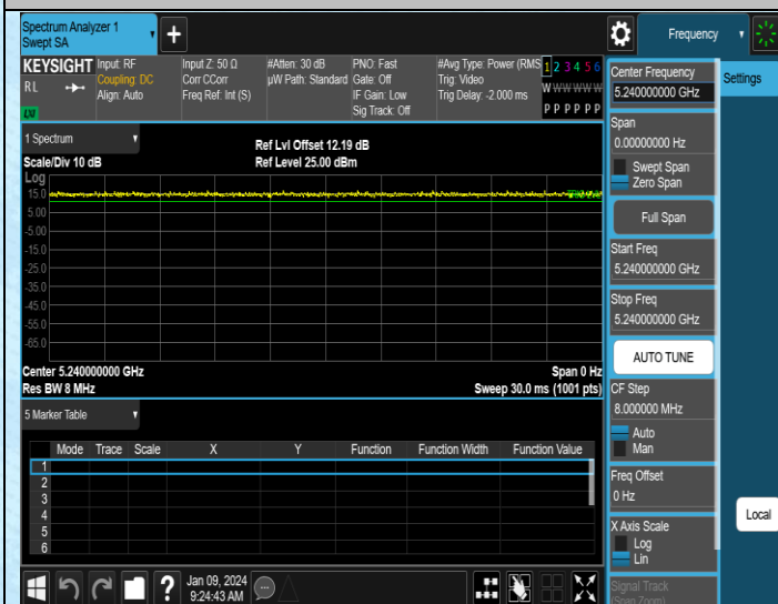
NTNV-11N20MIMO-Ant3-5240
