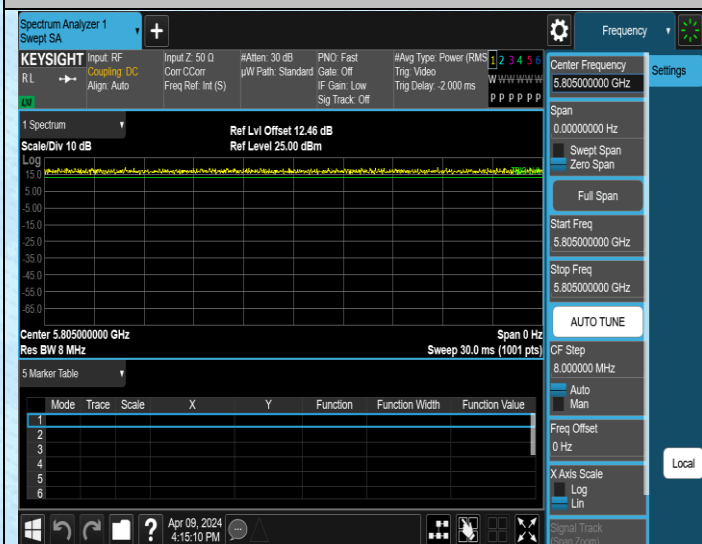
NTNV-11N20SISO-Ant3-5805
