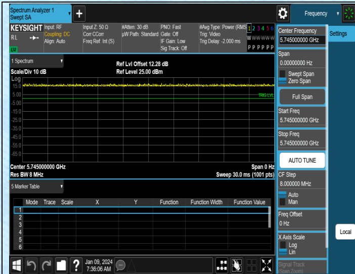
NTNV-11N20SISO-Ant3-5745
