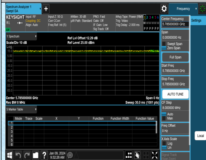
NTNV-11N20MIMO-Ant3-5785
