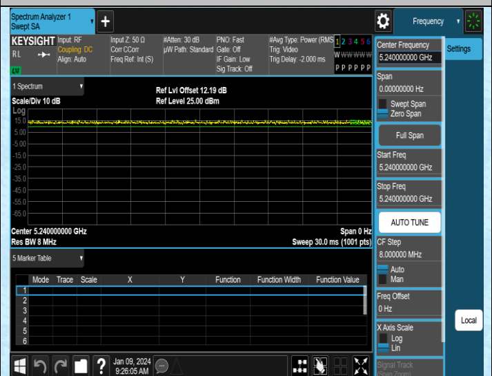
NTNV-11N20MIMO-Ant4-5240
