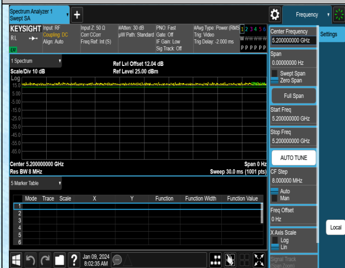
NTNV-11AC20SISO-Ant3-5200
