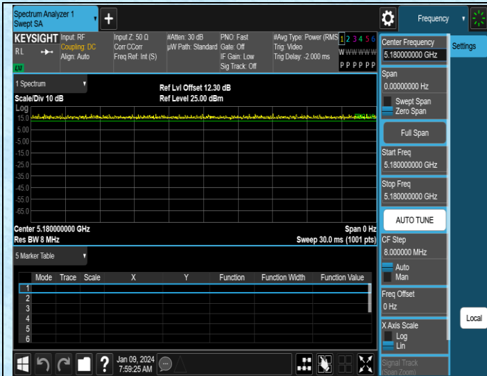
NTNV-11AC20SISO-Ant3-5180
