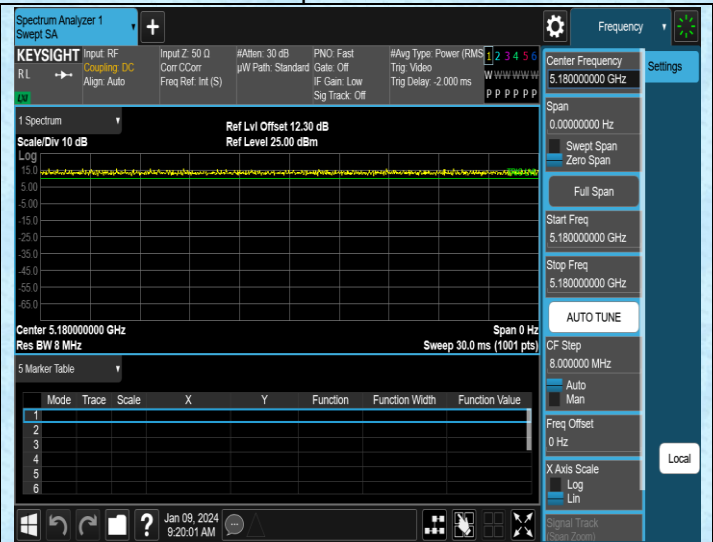
NTNV-11N20MIMO-Ant4-5180
