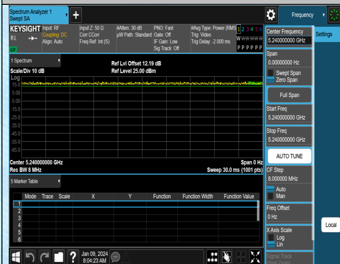
NTNV-11AC20SISO-Ant3-5240
