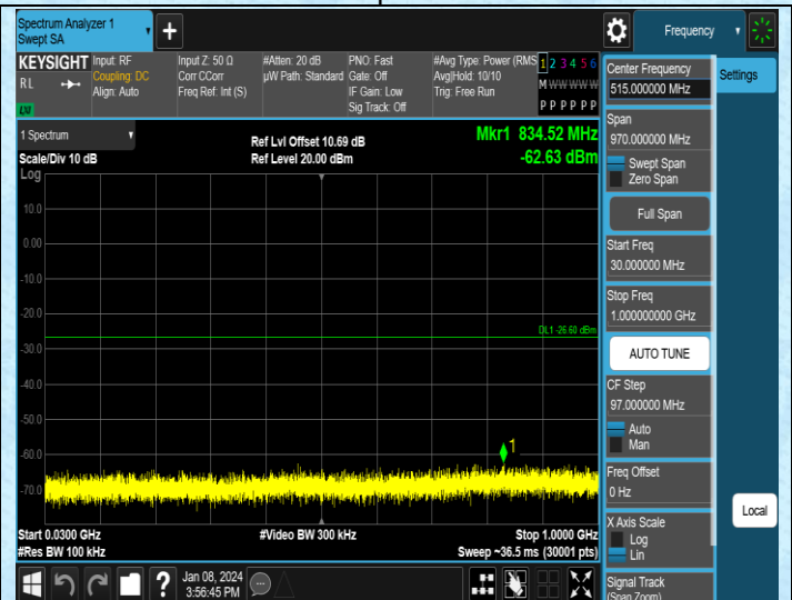
11N20MIMO-Ant3-2462-30~1000-PASS
