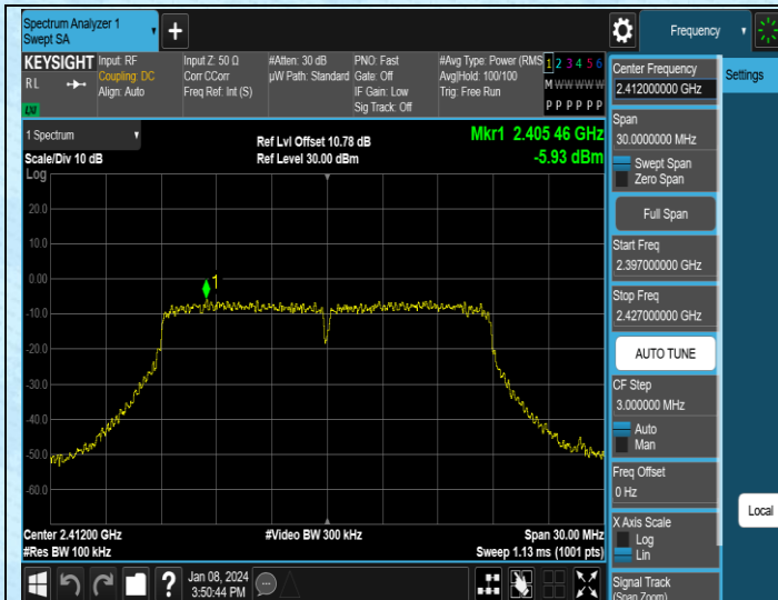
11N20MIMO-Ant3-2412-0~Reference-PASS
