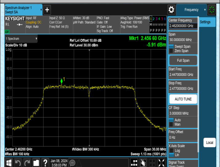
11N20MIMO-Ant4-2462-0~Reference-PASS
