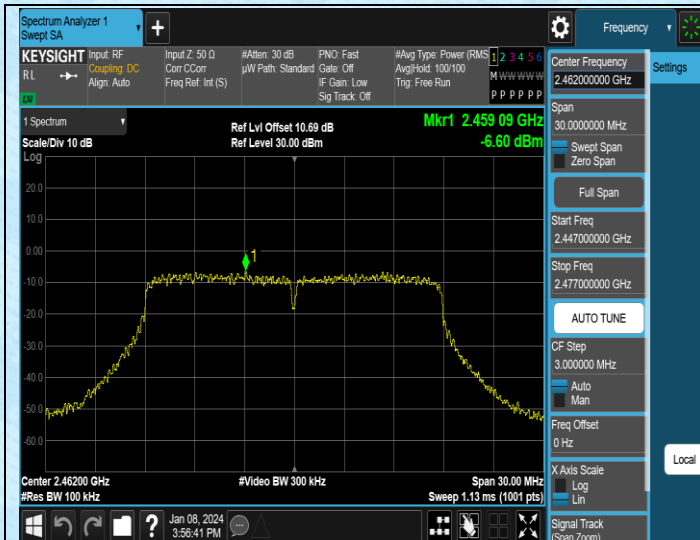
11N20MIMO-Ant3-2462-0~Reference-PASS
