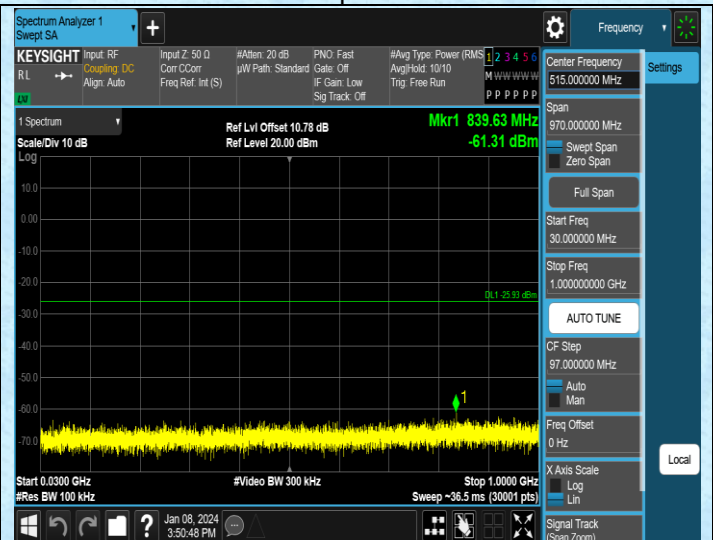
11N20MIMO-Ant3-2412-30~1000-PASS
