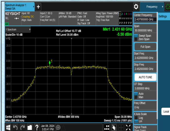
11N20MIMO-Ant3-2437-0~Reference-PASS
