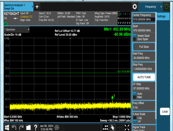
11N20MIMO-Ant3-2437-30~1000-PASS
