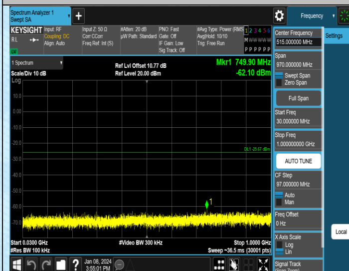
11N20MIMO-Ant4-2437-30~1000-PASS
