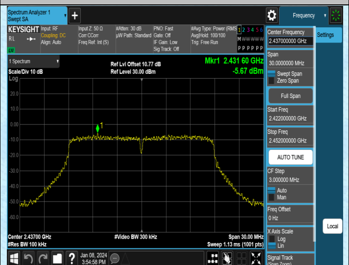
11N20MIMO-Ant4-2437-0~Reference-PASS
