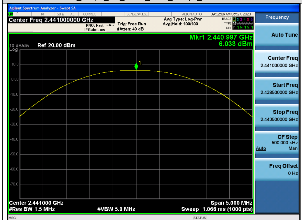
Test_Graph_BR_ANT1_2441_1Mbps_Peak Power
