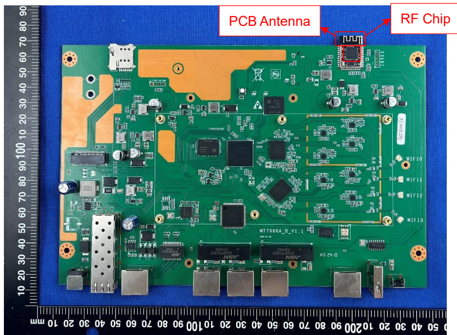
MAIN BOARD TOP VIEW (WITHOUT SHIELDING)
