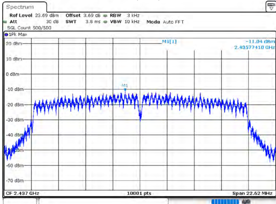
PSD NVNT 802.11n(HT20) 2437MHz Ant2
