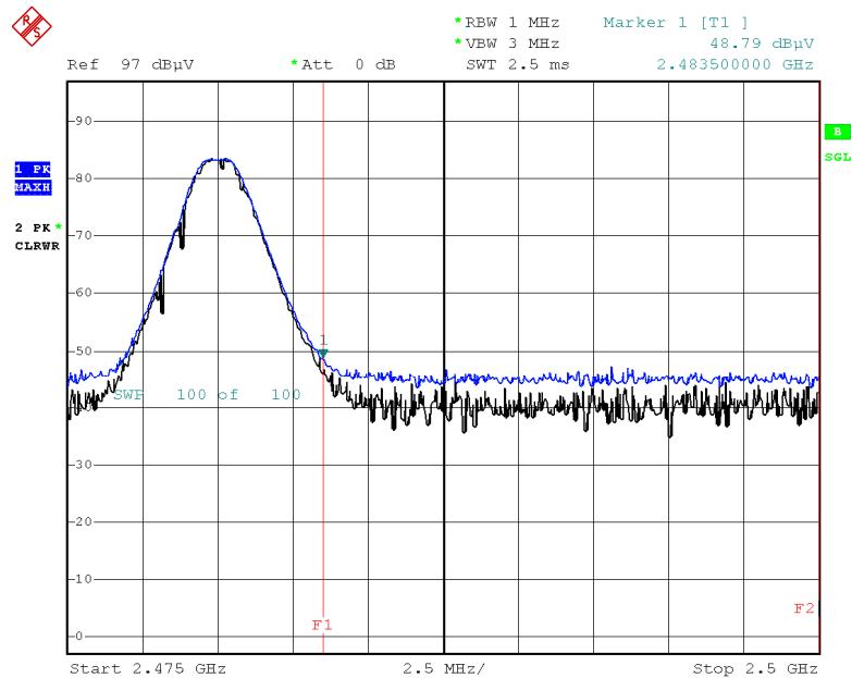
Radiated Restricted Band Edges plot – Peak Result (Ch.39, X-H)
