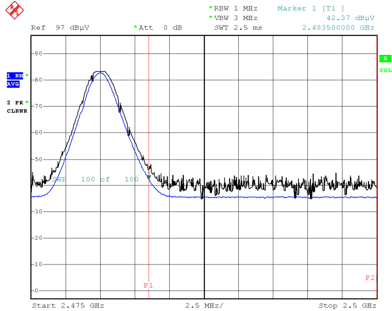
Radiated Restricted Band Edges plot – Average Result (Ch.39, X-H)
