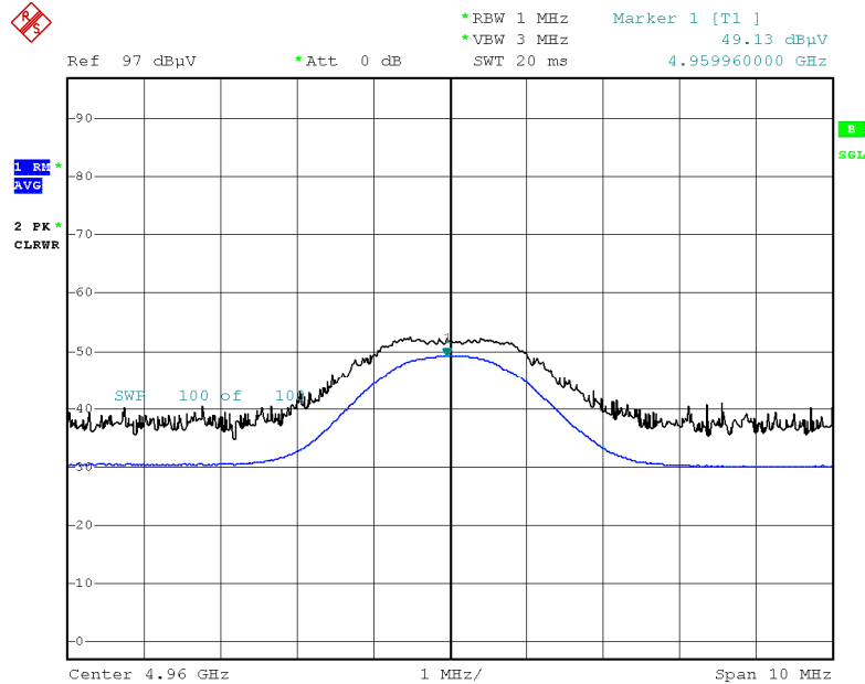
Radiated Spurious Emissions plot – Average Result (Ch.39 2nd Harmonic, Y-H)
