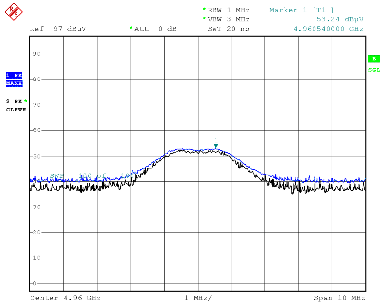
Radiated Spurious Emissions plot – Peak Result (Ch.39 2nd Harmonic, Y-H)
