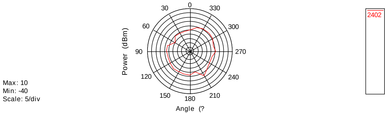
2D(Y-Z Plane) RDA5875Y Antenna Gain Free Space-2402MHz
