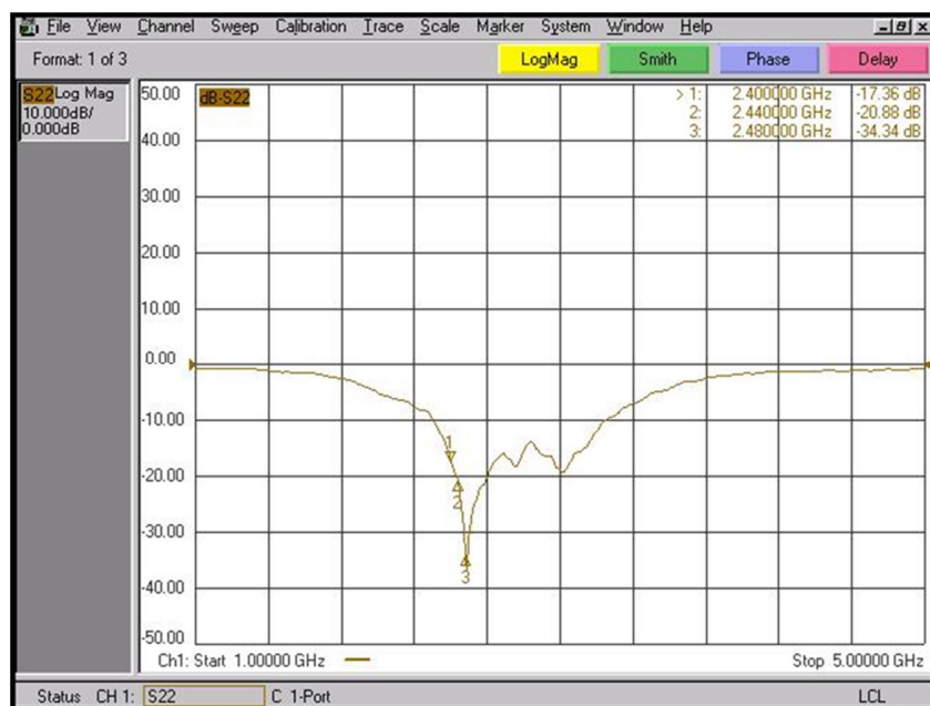
S22 measurement
