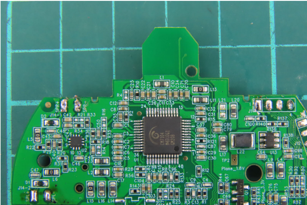
(38) EUT Photo
