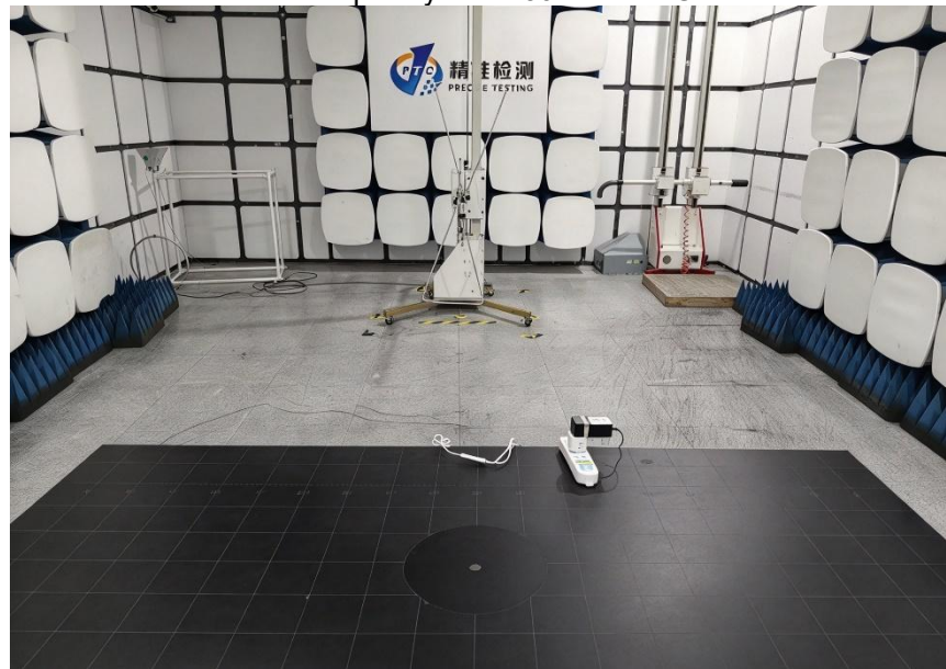
Radiated Spurious Emissions Test Frequency From 30MHz to 1GHz
