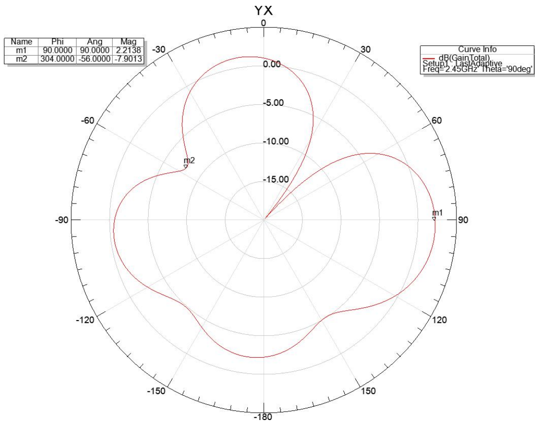
Radiation Pattern 2
