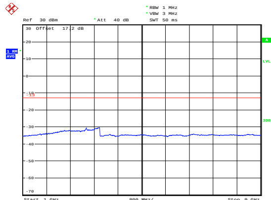
NB-IOT Band 5 CH-High 1GHz-9GHz
