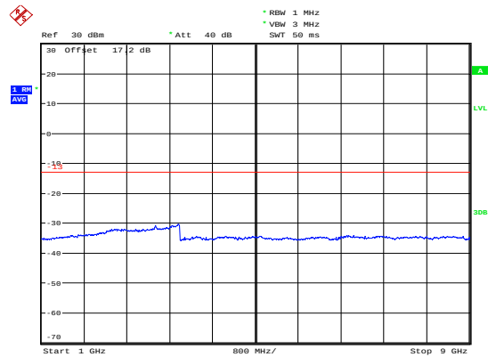
NB-IOT Band 5 CH-Low 1GHz-9GHz
