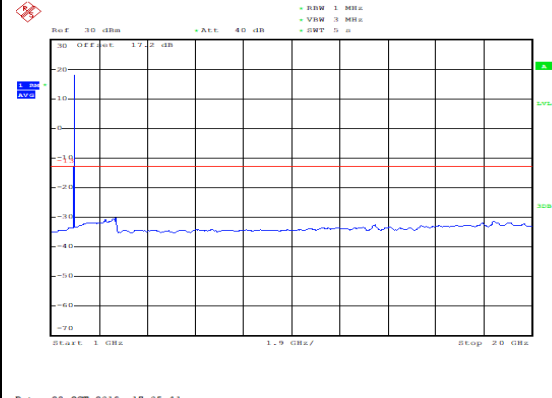
LTE Band 2 1.4MHz CH-High 1GHz ~20GHz
