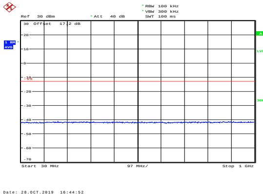
LTE Band 2 1.4MHz CH-High 30MHz~1GHz
