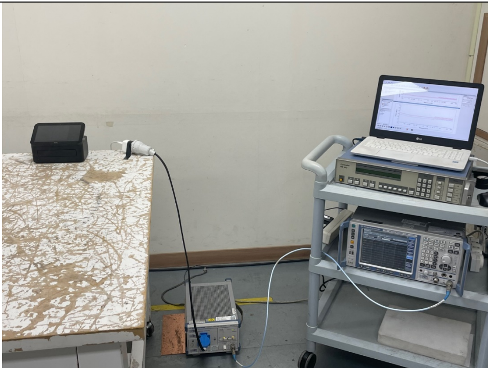
Conducted Emissions
