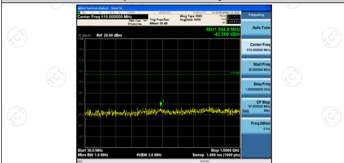
Band66-5MHz-QPSK-132647-1RB#0-Range2:1000~20000MHz
