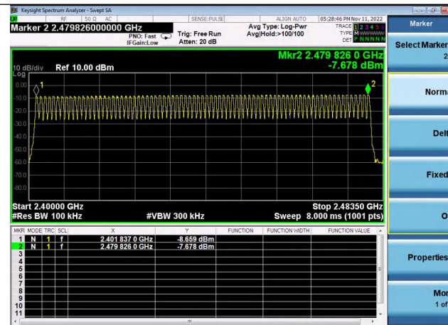
GFSK Modulation
