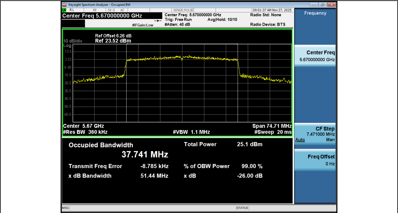
-26BW_NVNT_ANT2_802_11ax(HE40)_5670
