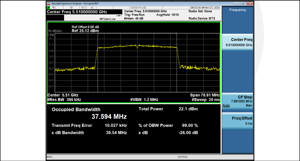
-26BW_NVNT_ANT2_802_11ax(HE40)_5510
