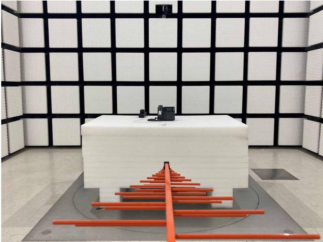
Radiated Emission Below 1GHz View POE Power
