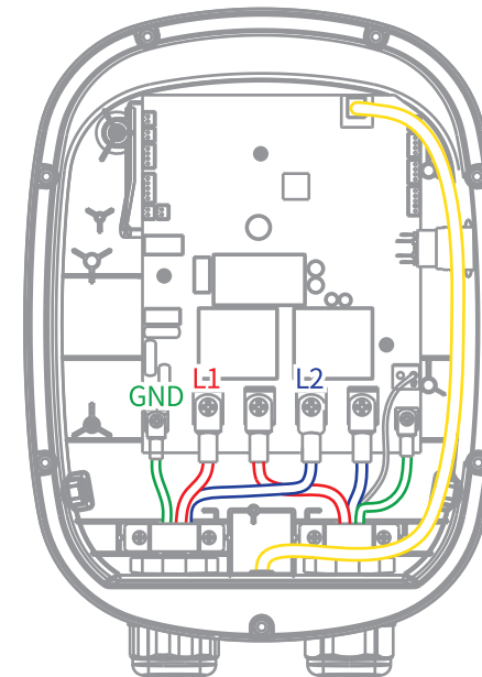
Without an ammeter
