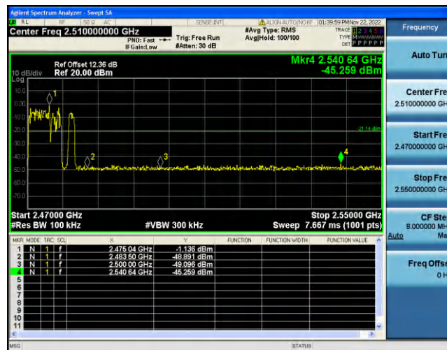
3DH5-Ant1-High-Hop_2480--1.14
