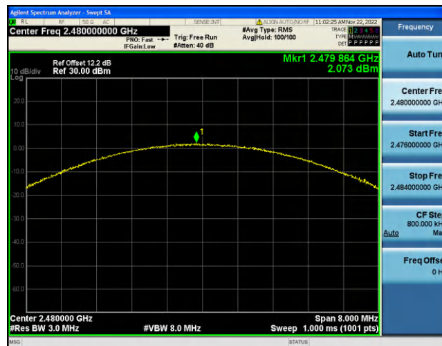
3DH5-Ant1-2480
