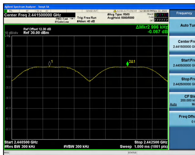
2DH5-Ant1-Hop
