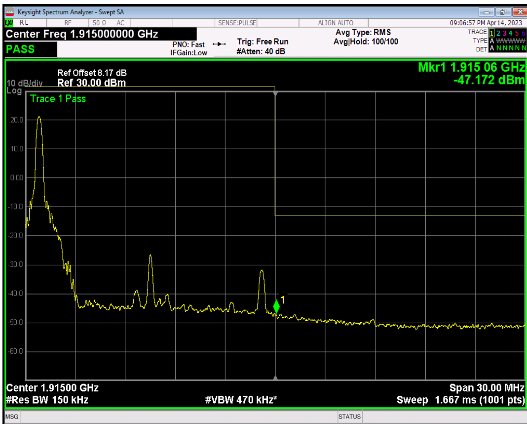
Band25 QAM16 BW=15MHz Channel=26615 RB Size=1 Position=#Max
