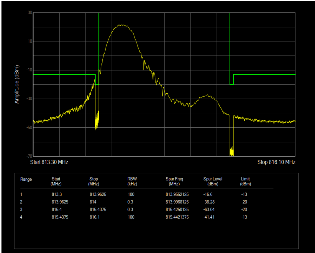
Band26(814-824) QPSK BW=1.4MHz Channel=26697 RB Size=1 Position=#Max
