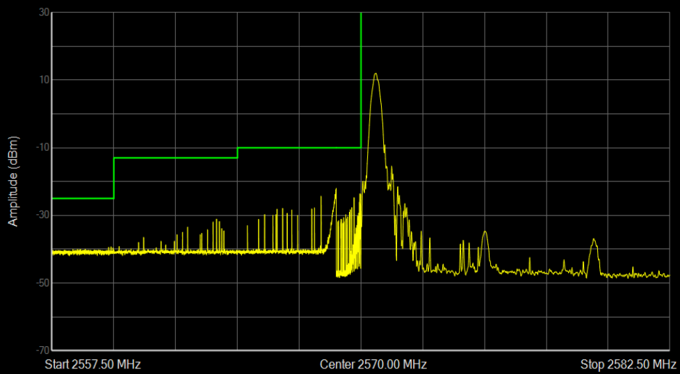
Band38 QAM16 BW=10MHz Channel=37800 RB Size=1 Position=#0
