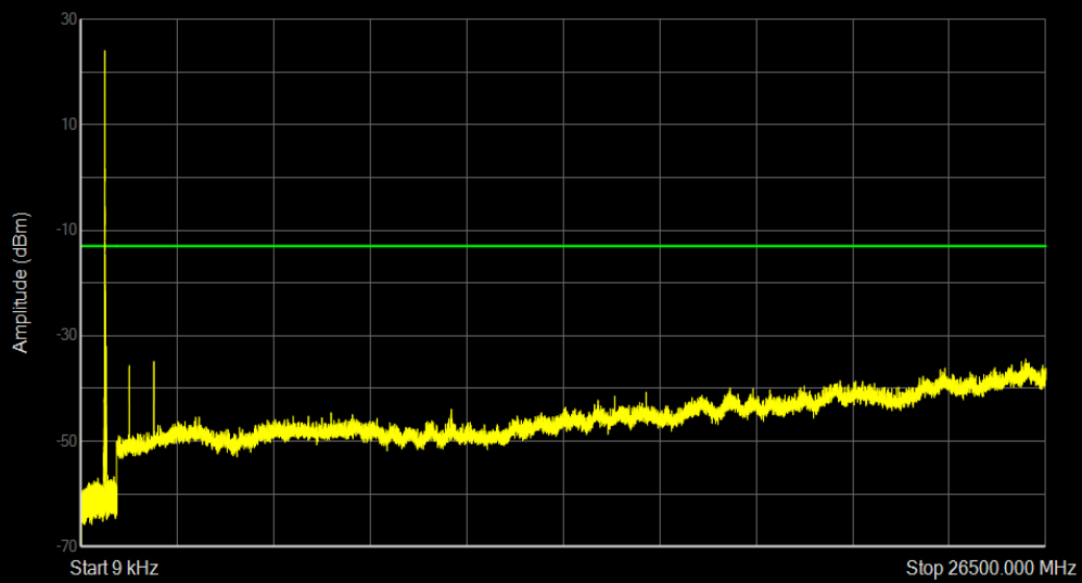
Band71 QPSK BW=20MHz Channel=133322 RB Size=1 Position=#0
