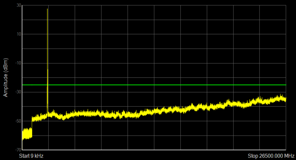
Band41 QPSK BW=15MHz Channel=40315 RB Size=1 Position=#0
