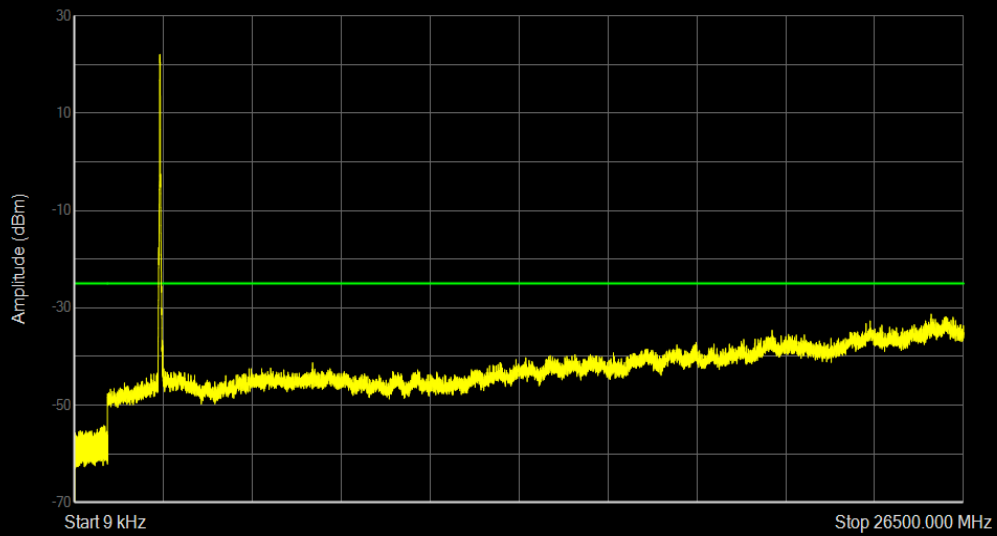
Band41 QAM16 BW=20MHz Channel=40340 RB Size=100 Position=#0
