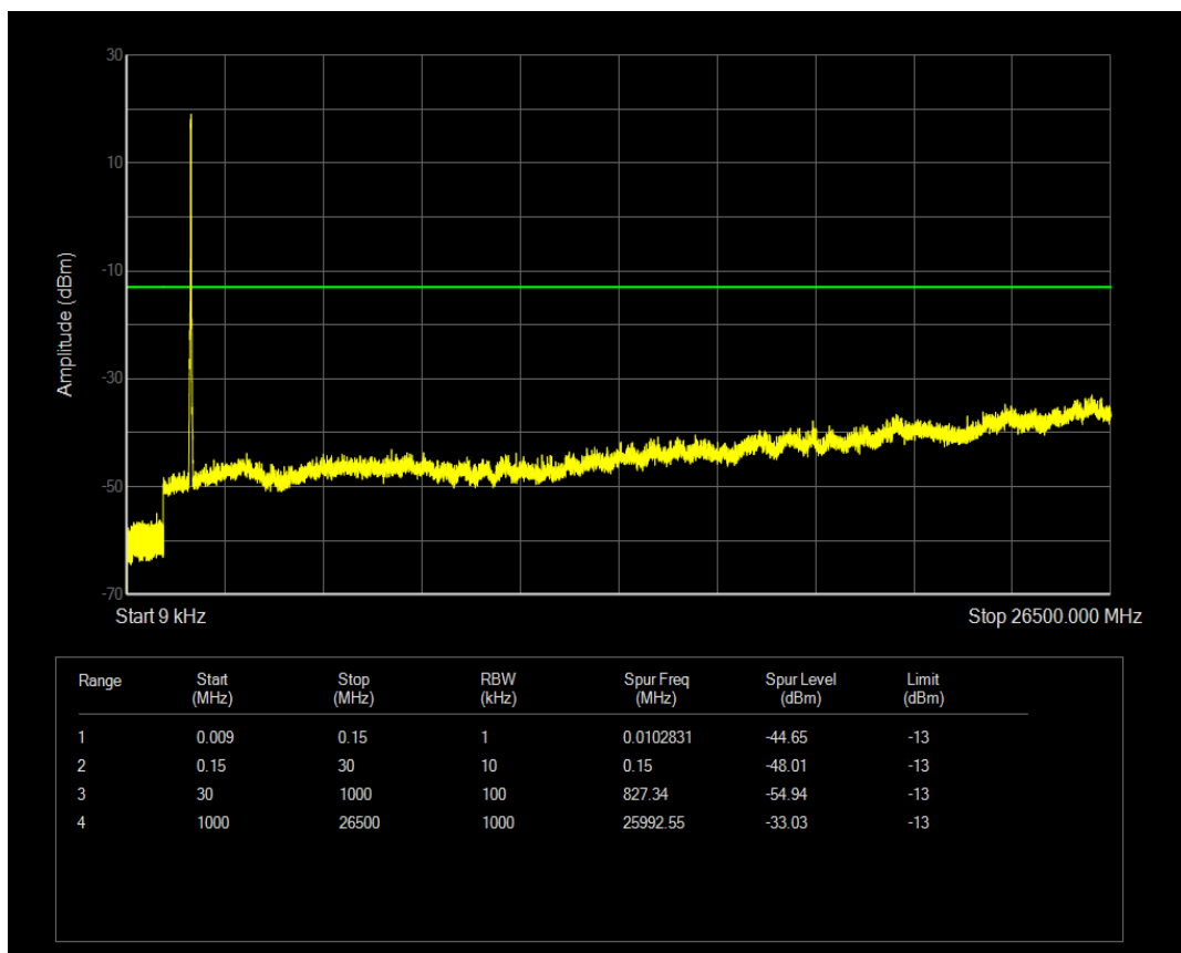
Band41 QPSK BW=5MHz Channel=40265 RB Size=1 Position=#0
