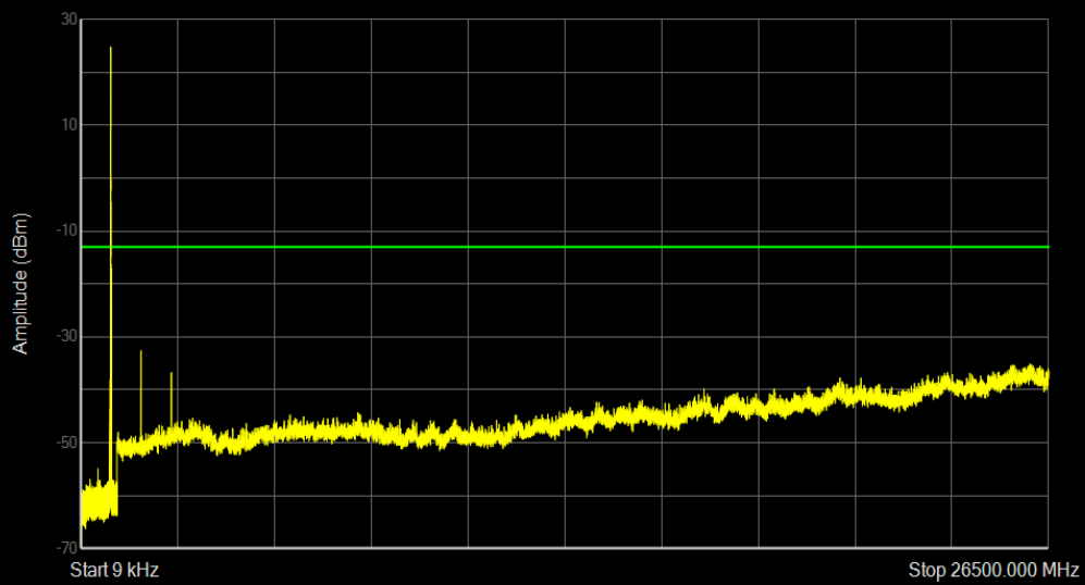
Band26b QAM16 BW=15MHz Channel=26915 RB Size=1 Position=#0
