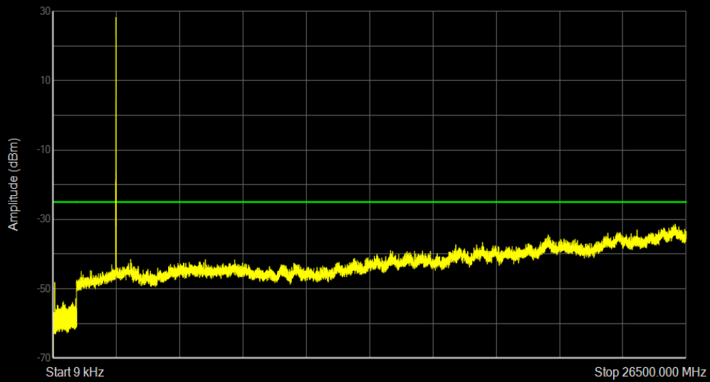
Band41 QAM16 BW=5MHz Channel=41215 RB Size=1 Position=#0
