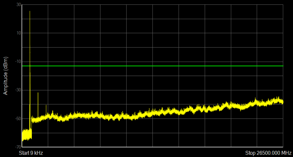
Band26b QAM16 BW=15MHz Channel=26865 RB Size=1 Position=#0
