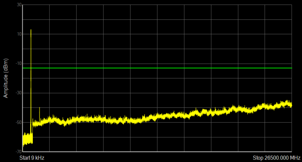
Band26b QPSK BW=10MHz Channel=26990 RB Size=50 Position=#0
