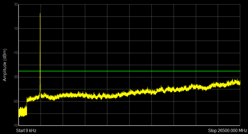
Band41 QAM16 BW=15MHz Channel=40620 RB Size=75 Position=#0
