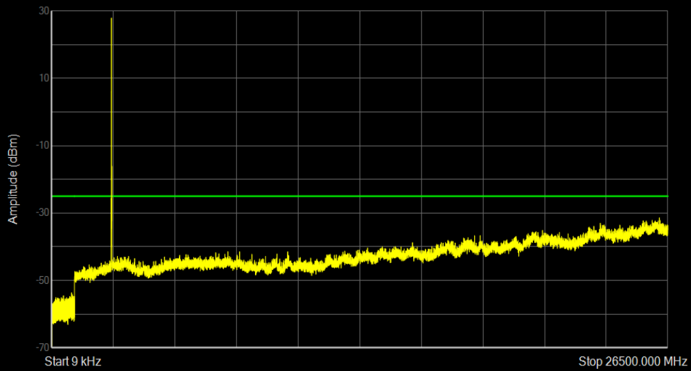
Band41 QAM16 BW=10MHz Channel=40620 RB Size=1 Position=#0
