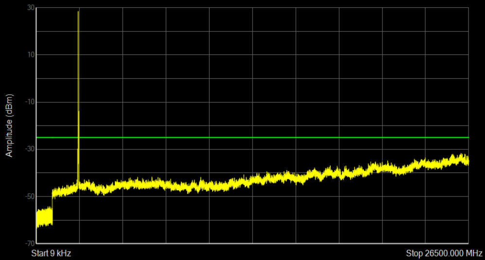
Band41 QAM16 BW=15MHz Channel=40620 RB Size=1 Position=#0
