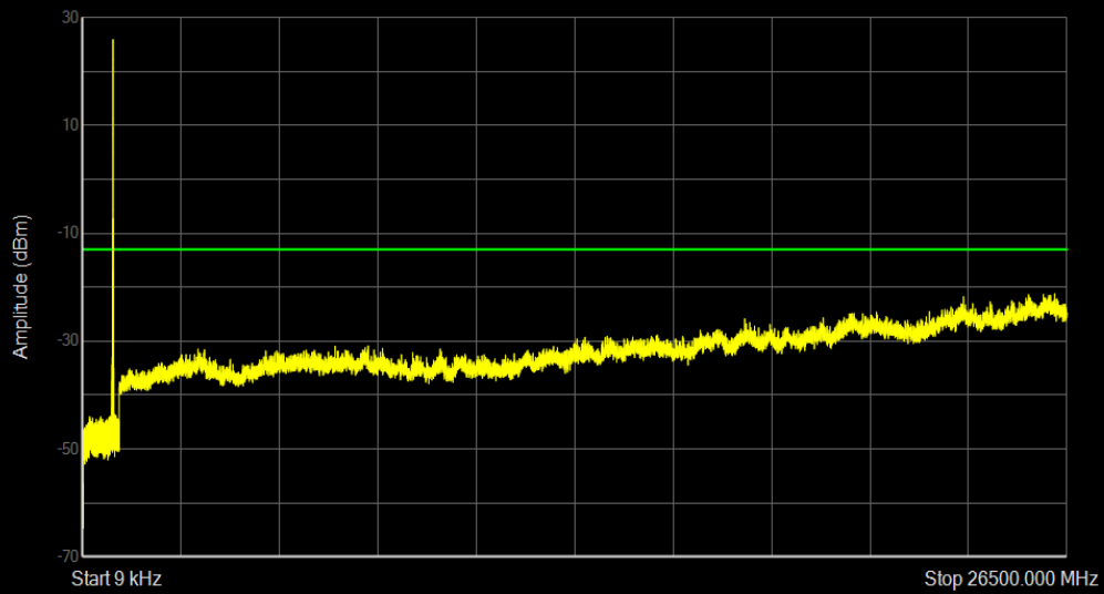
Band5 QAM16 BW=3MHz Channel=20525 RB Size=1 Position=#0
