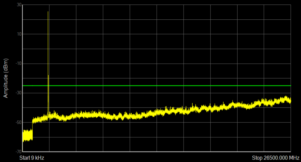
Band41 QAM16 BW=20MHz Channel=40140 RB Size=1 Position=#0
