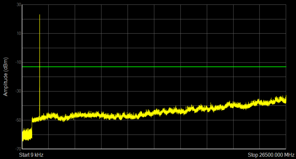
Band66 QPSK BW=5MHz Channel=132647 RB Size=25 Position=#0
