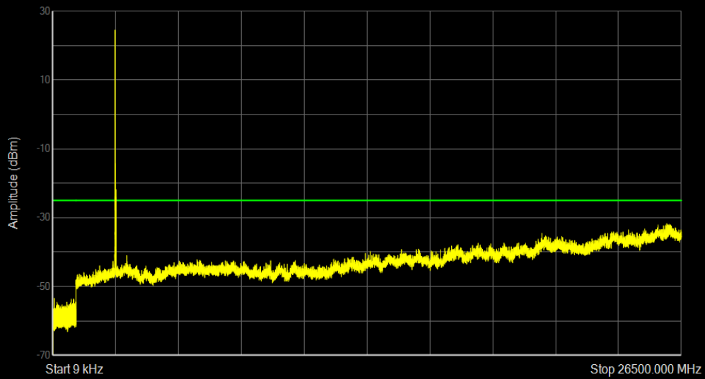
Band41 QPSK BW=10MHz Channel=41190 RB Size=1 Position=#0
