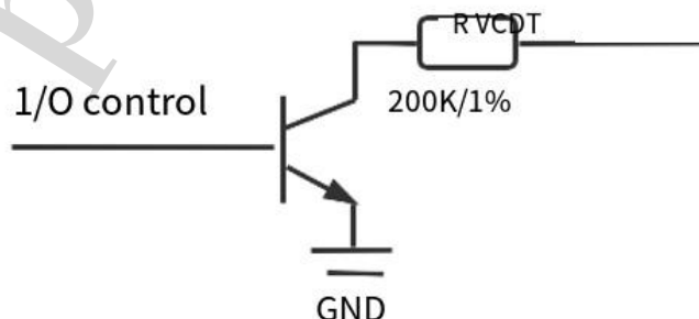
VCDT partial voltage shunt resistance design
