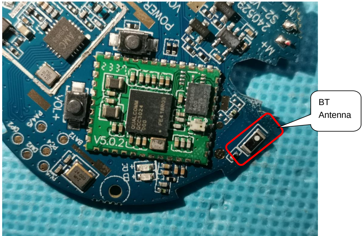
INTERNAL VIEW OF EUT (FIGURE 4)
