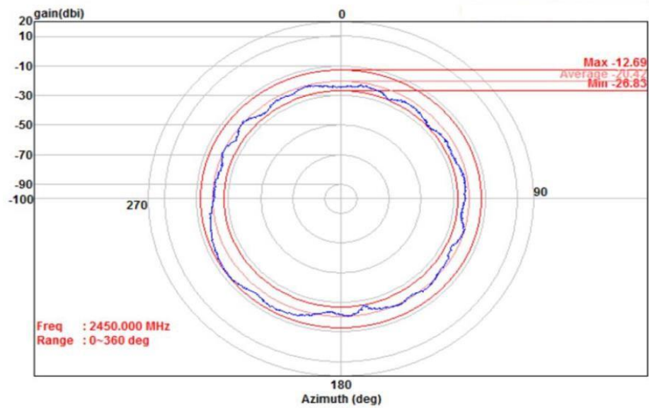
FIGURE 3-2: ANTENNA 3D RADIATION PATTERN @2450 MHz
