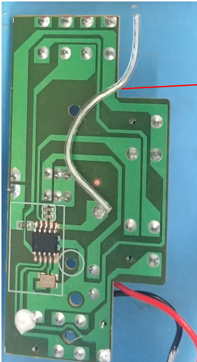
Antenna Photo & Length (mm)
