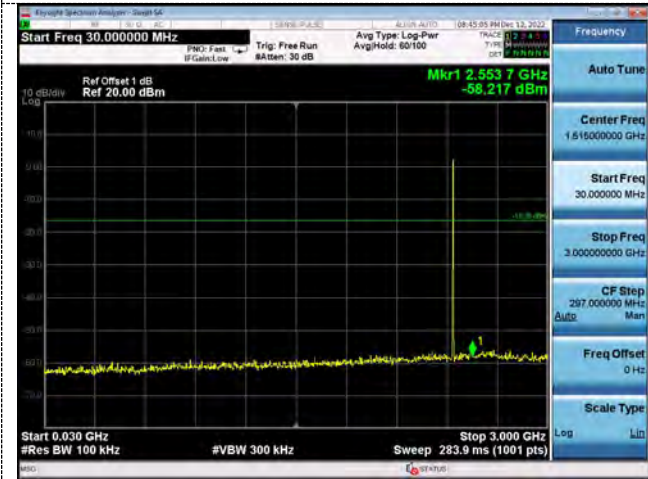
30MHz-3G
