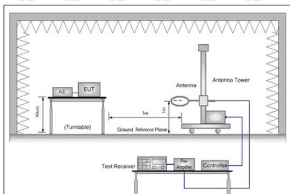
Figure 1. Below 30MHz
