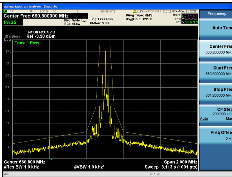
660.8MHz Emission Mask
