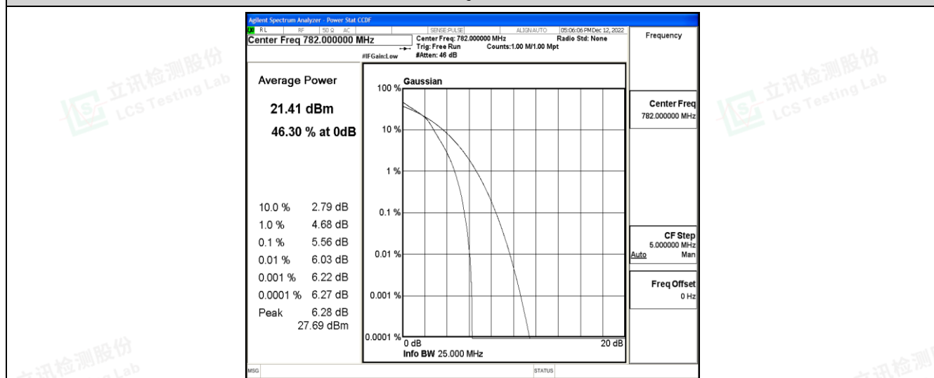
Band13-5MHz-16QAM-23255-25RB#0
