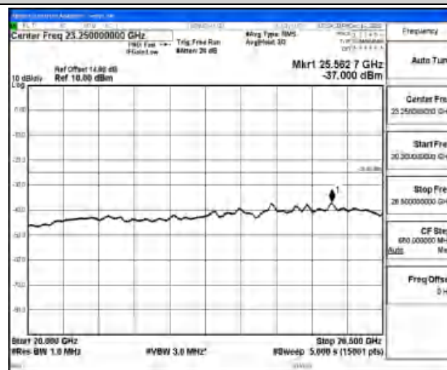
Band41-20MHz-16QAM-41490-1RB#0-Range6:20000~26500MHz
