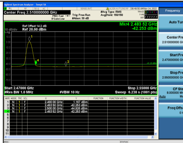
BLE_2M-Ant1-High-2480-AV-2483.500
