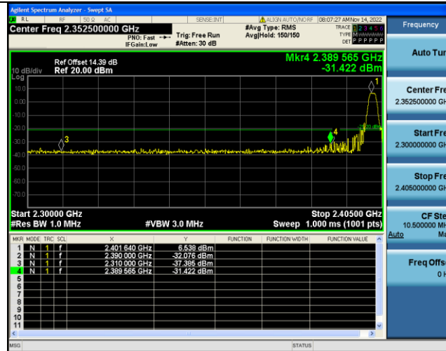
BLE_2M-Ant1-Low-2402-AV-2390.000
