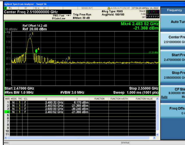
BLE_1M-Ant1-High-2480-AV-2483.500
