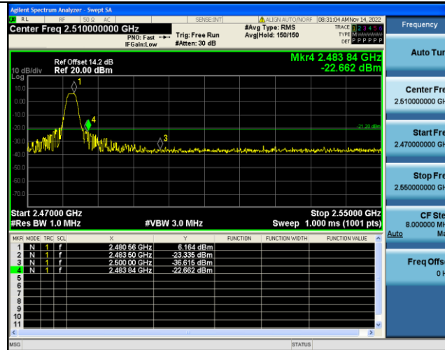
BLE_2M-Ant1-High-2480-AV-2483.500
