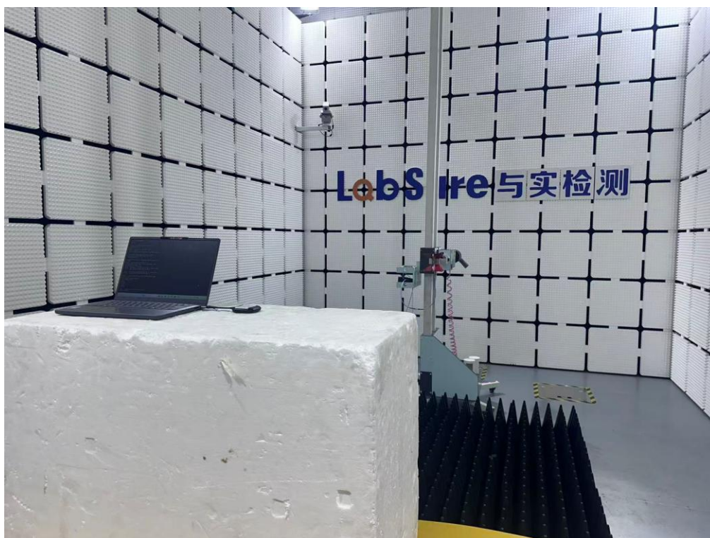
RSE Setup for 1GHz-18GHz
