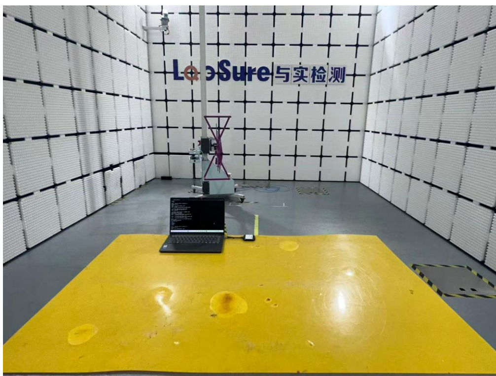
RSE Setup for 30MHz-1GHz
