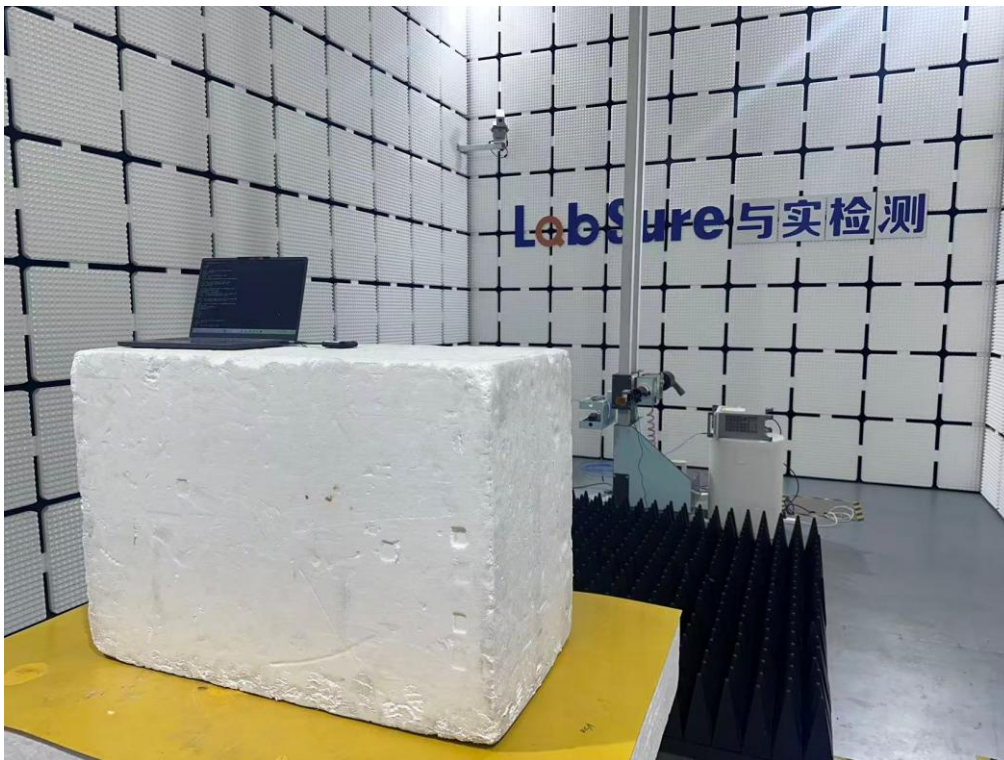
RSE Setup for 18GHz-40GHz
