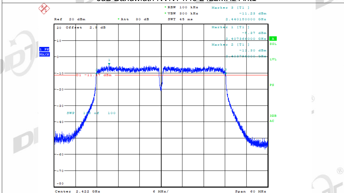
-6dB Bandwidth NVNT n40 2422MHz Ant1
