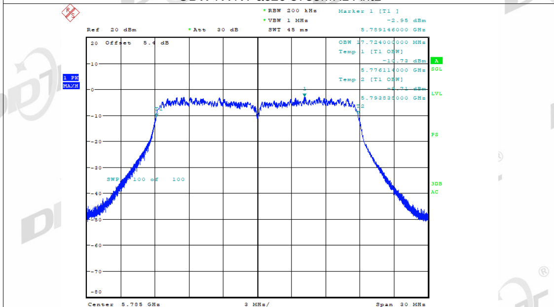
OBW NVNT ac20 5785MHz Ant1
