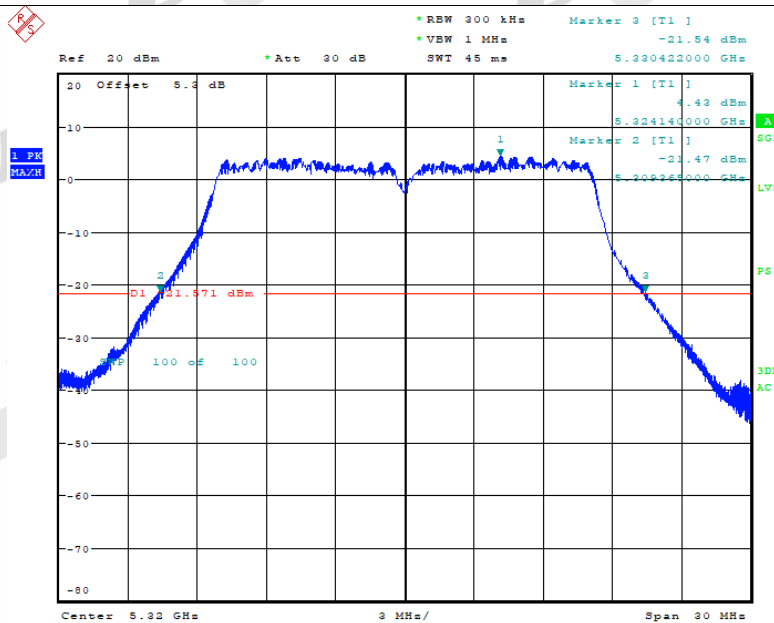
-26dB Bandwidth NVNT a 5320MHz Ant1
