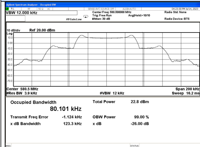
Channel 1 / 580.5 MHz
