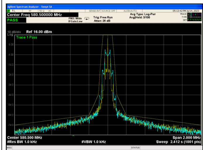
Channel 1 / 580.5 MHz
