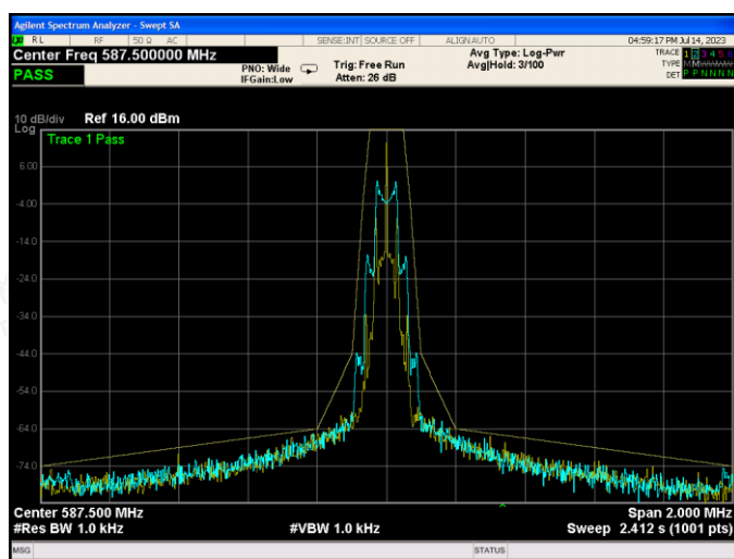
Channel 8 / 587.5 MHz
