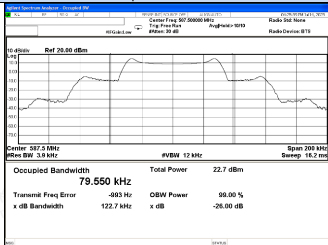
Channel 8 / 587.5 MHz
