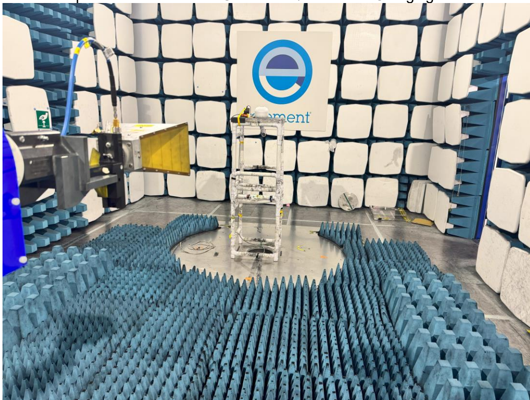
Radiated Spurious Emissions > 1GHz – Hub / Handheld Charging in Hub:
