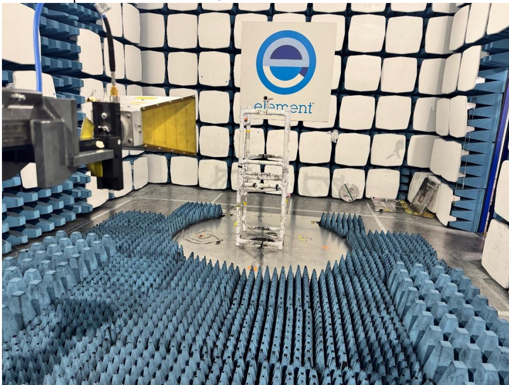
Radiated Spurious Emissions > 1GHz – Handheld:
