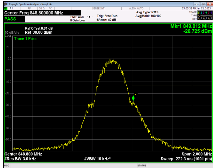
GPRS850 Channel=251
